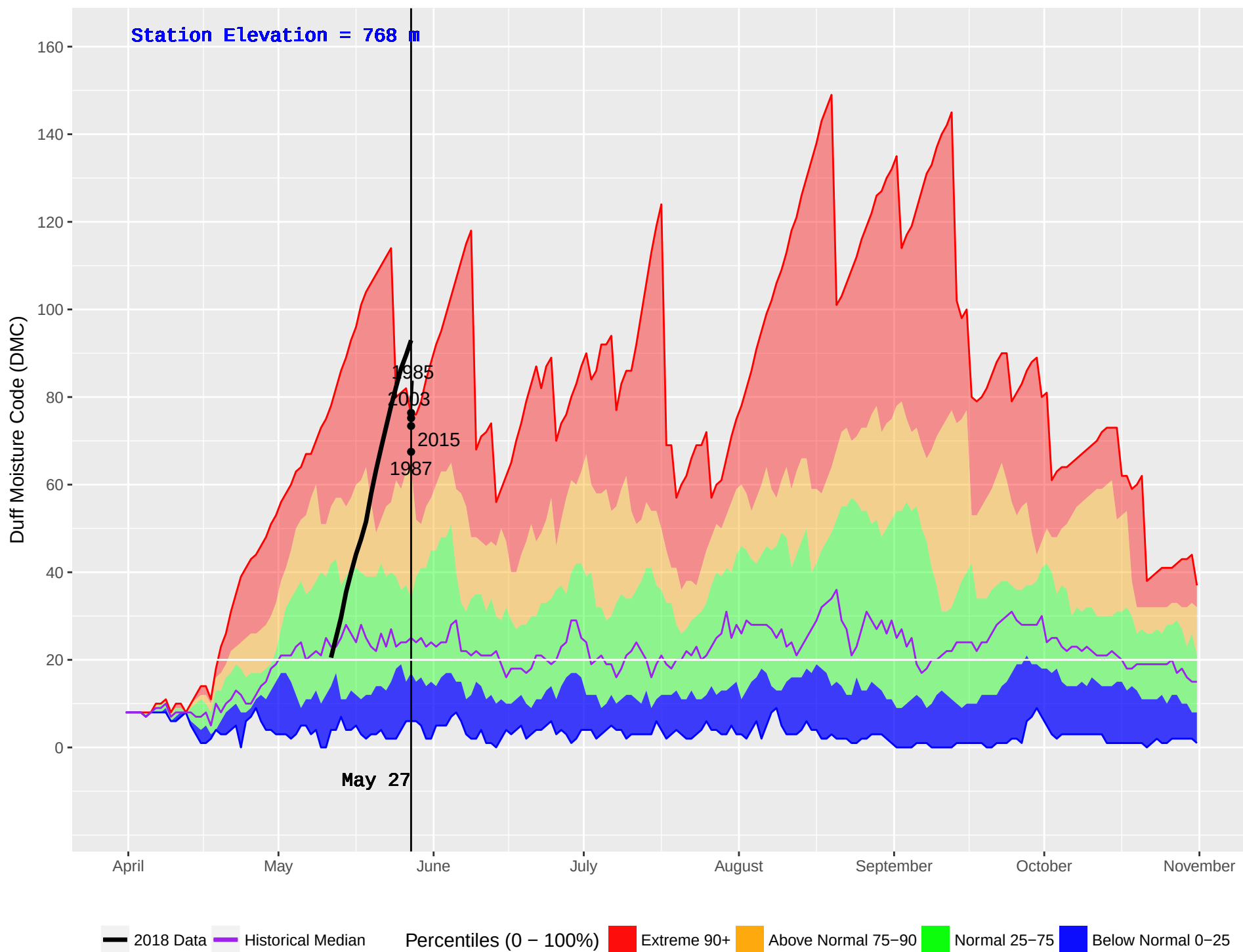
GRAHAM (124) : Historical (1979–2016) and Current (2018) Noon Duff Moisture Code (DMC)
